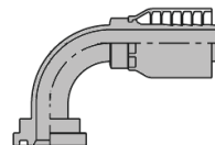
SAE Code 62 Split Flange 90° Elbow (FHB)
