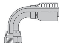
DKO Female Swivel, Heavy Duty, 90° Elbow (DSB)
