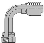
Female JIC/SAE 37° Swivel 90° Long Drop Elbow (FJC)
